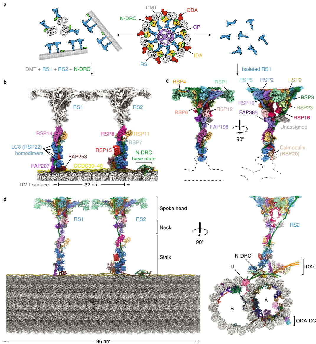
Fig. 1 | Structures of radial spokes on and off doublet microtubules. a , Schematic representation showing biochemical fragmentation of the Chlamydomonas axoneme (viewed in cross-section; center) into mechanoregulator-bound doublet microtubules (left) and isolated radial spokes (right). The axoneme consists of a central pair of microtubules (CP, purple) surrounded by doublet microtubules (DMT; gray) bound by radial spokes (RS; blue), nexin–dynein regulatory complexes (N-DRC; green), inner dynein arm (IDA; yellow) and outer dynein arm (ODA; red). b , Composite density map for on-doublet RS1 and RS2. The maps of the stalks are colored by subunit. The neck and spoke head, which are less well resolved, are colored gray. c , Orthogonal views of a composite density map for isolated RS1 with the map colored by subunit. Dashed lines indicate the positions of the stalks and doublet microtubule, which are not present in the reconstruction. d , Orthogonal views of an atomic model for the 96-nm repeat of the doublet microtubule. The model combines atomic models of the doublet-bound stalks of RS1 and RS2, and the stalk, neck and spoke head of isolated RS1 with the model of the doublet microtubule (PDB 6U42) 21 . Individual subunits are colored as in b,c . In b,d , the minus (–) and plus (+) ends of the doublet microtubule are indicated at the ends of the scale bar. The inner junction (IJ) and ODA docking complex (ODA-DC) are labeled.
