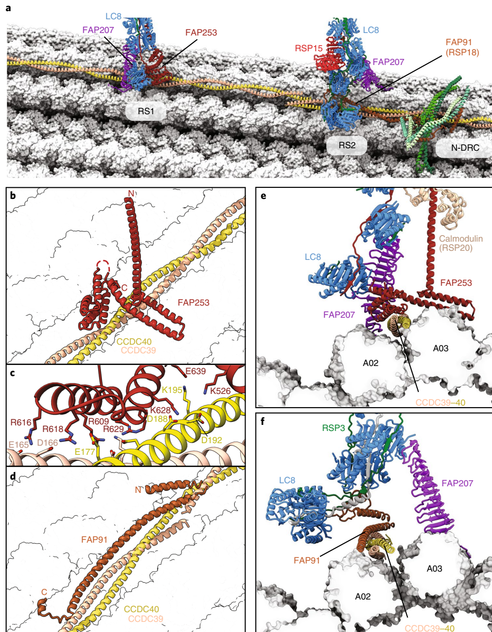
Fig. 2 | Structural basis for the microtubule docking and longitudinal periodicity of radial spokes. a , Overview showing the bases of RS1 and RS2 bound to the doublet microtubule. The radial spoke subunits (LC8, FAP91, FAP207, FAP253 and RSP15), the CCDC39–40 molecular ruler, and the subunits of the N-DRC base plate are shown as cartoons. Tubulin is shown in surface representation. b , The binding site for RS1 is determined by recognition of CCDC39–40 by FAP253. c , Zoomed-in view showing that the interface between FAP253 and CCDC39–40 is dominated by a network of salt bridges. d , The binding site for RS2 is determined by FAP91 (RSP18), which forms a triple coiled coil with CCDC39–40. e , Cross-section view of the RS1–doublet microtubule interaction showing recognition of CCDC39–40 by FAP253. FAP207 bridges LC8 with protofilament A02. f , Cross-section view of the RS2–doublet microtubule interaction showing recognition of CCDC39–40 by FAP91. FAP207 bridges LC8 with protofilament A03.
