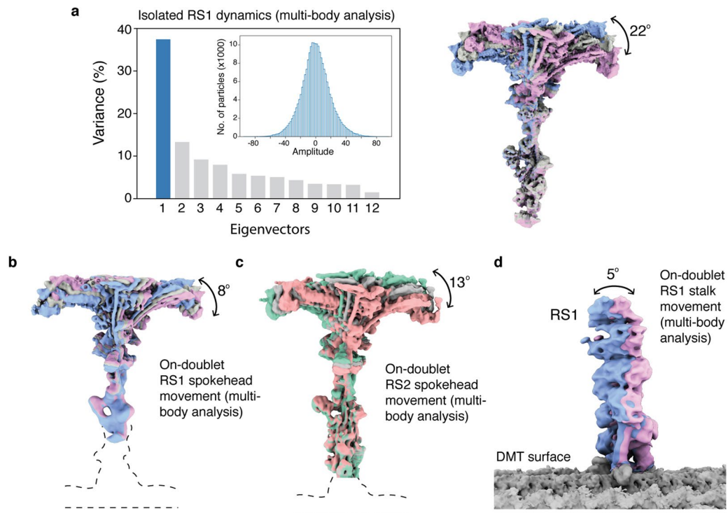
Extended Data Fig. 9 | Dynamics of radial spokes by multi-body analysis. a , Multi-body analysis of isolated RS1. Left, the contributions of all eigenvectors to the variance. The first eigenvector accounts for 37% of all variability. Inset, the unimodal histogram of amplitudes along the first eigenvector indicates continuous motion. Right, the density maps at the extremes and middle show the same tilting of the spoke head relative to the stalk as observed by the neural-network approach in Fig. 6a. b , Multi-body analysis of on-doublet RS1 shows the same direction of spoke head tilt as isolated RS1. c , Multi-body analysis of on-doublet RS2 shows that the spoke heads of both radial spokes tilt in similar directions to similar extents. d , Multi-body analysis of the movement of the RS1 stalk with respect to the doublet microtubule (DMT) surface.
