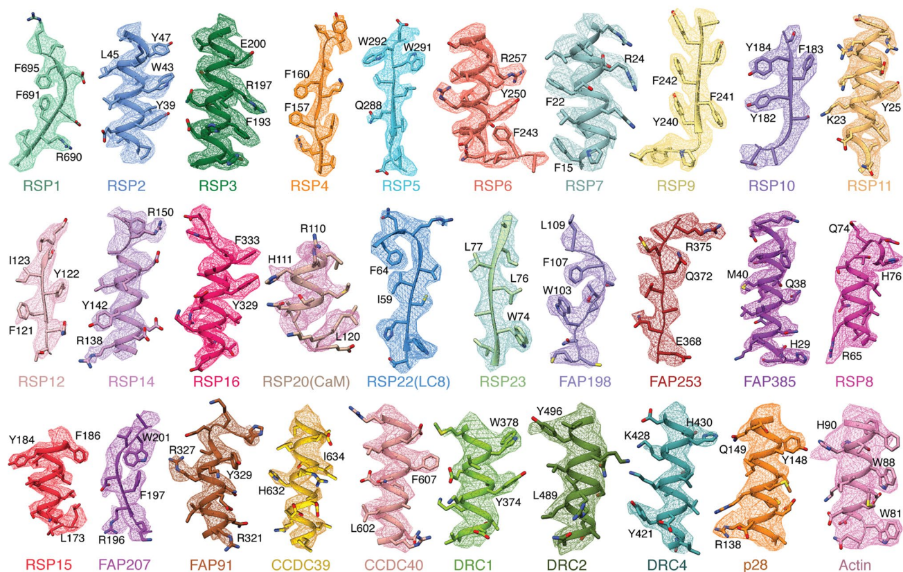
Extended Data Fig. 3 | Map quality. Examples of map density for all 30 non-tubulin proteins identified in this study. The first 19 proteins show density from isolated RS1 contoured at 0.009–0.013. The remaining 11 proteins (starting from RSP8) show density from on-doublet maps contoured at 0.020–0.031. Landmark residues are labeled. Note that the sidechains of RSP20 (calmodulin) and RSP8 are not well resolved and are truncated in the deposited model.
