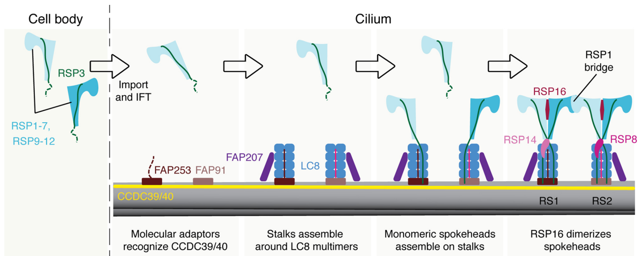
Extended Data Fig. 8 | Model of radial spoke assembly. Proposed model of radial spoke assembly. Monomeric spoke head lobes, comprising RSP1-7 and RSP9-12, assemble in the cell body 28,34-36 before being imported into the cilium by intraflagellar transport (IFT) 34,74 . In the cilium, the axonemal doublet microtubules are bound by the CCDC39-40 coiled coil. Specific sequences within the coiled coil are recognized by molecular adaptors FAP253 and FAP91 that establish the binding sites for RS1 and RS2. These molecular adaptors recruit LC8 and FAP207, although the arrangement of these elements is different in the two stalks. RSP3 in the precursor binds the LC8 multimers (Fig. 4b), helping dock the spoke head lobe onto the preassembled stalks. Two lobes can bind a single stalk. Binding of RSP16 is presumably a relatively late step that dimerizes the lobes 28 . At a similar time, RS-specific proteins bind; RSP14 to RS1 and RSP8 to RS2.
