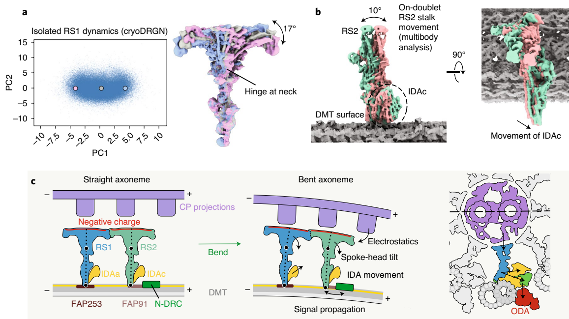
Fig. 6 | Molecular basis for the control of IDA motor activity by mechanical signals. a , Conformational dynamics of isolated RS1 inferred from deep neural networks. Left, principle component (PC) analysis projection of latent space. Density maps were generated at three points along PC1. Right, density maps generated from these three points were aligned on the stalk and show tilting of the spoke head relative to the stalk. The hinge lies in the neck. b , Multibody analysis of the movement of the RS2 stalk and IDAc with respect to the DMT surface. The DMT, RS2 and IDAc were separately masked and treated as individual bodies free to move relative to one another. Movement of IDAc corresponds with the movement of the RS2 stalk. c , A model for mechanoregulation of ciliary motility. As the axoneme bends, the projections of the CP are brought closer to the spoke heads. An increase in the electrostatic force with decreasing distance causes the radial spoke to tilt at two hinge points (indicated with black circles). As the movement of IDAc is coupled to the movement of RS2, tilting of the radial spoke changes the orientation of the IDA. IDAa may likewise be coupled to the movement of RS1. Signals may propagate from RS2 to N-DRC through FAP91 and the CCDC39–40 coiled coil and from the N-DRC to the ODAs via the outer-inner dynein linkers 26 .
