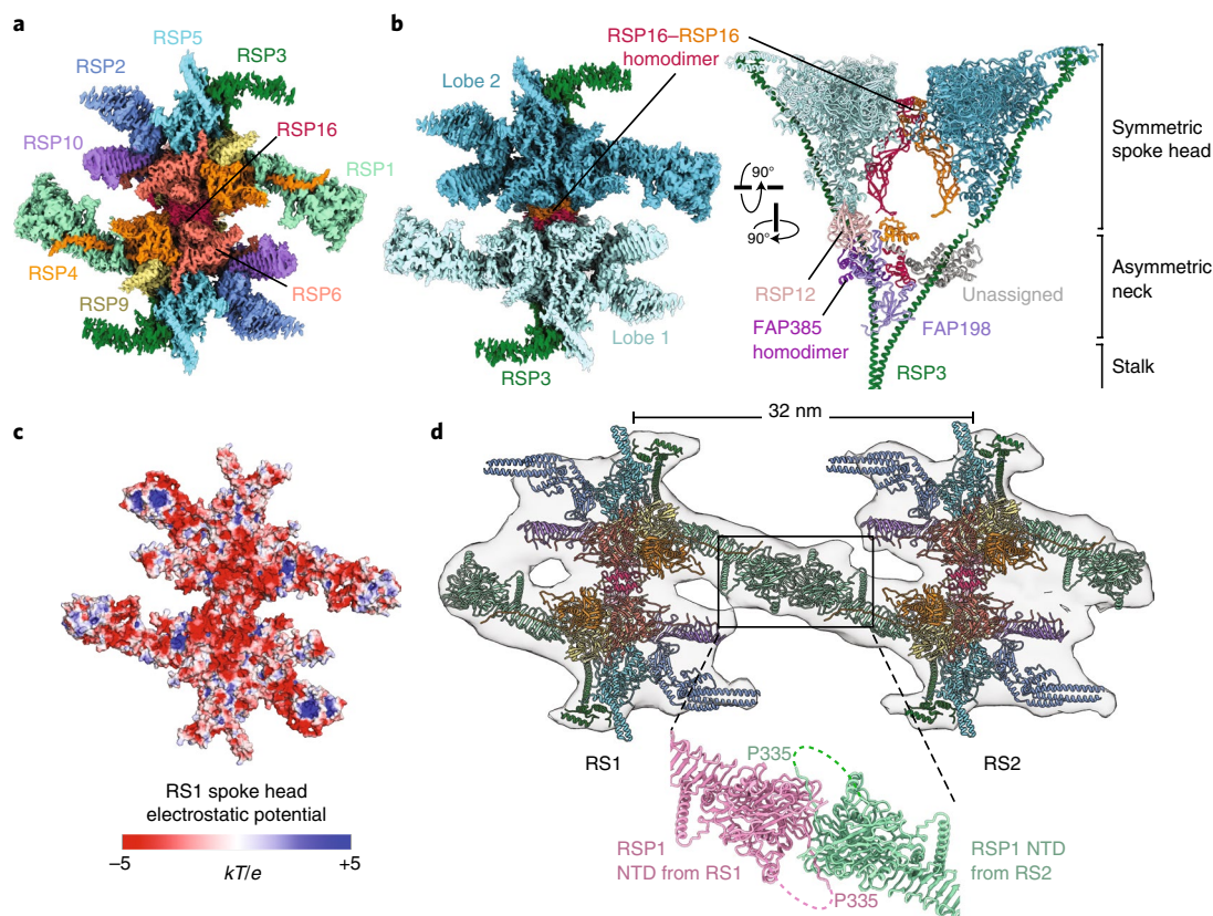
Fig. 3 | Structure of the radial spoke head. a , View of the top of the radial spoke head. Composite map colored by subunit. b , Two views of the radial spoke head. The two symmetric lobes of the spoke head (colored different shades of blue) are dimerized by a homodimer of RSP16 and flanked by the \alpha -helices of RSP3. The symmetric spoke head sits on a V-shaped asymmetric neck containing FAP198, FAP385, RSP12 and the N-terminal domains of RSP16. c , Atomic model of the radial spoke head colored by electrostatic potential. d , Atomic models of the radial spokes docked into an isosurface rendering of the subtomogram average of the Chlamydomonas axoneme (EMD-6872). The two radial spokes interact through the N-terminal domains (NTDs) of RSP1. Inset shows the model of the on-doublet interaction between the NTDs of RSP1 from RS1 and RS2.
