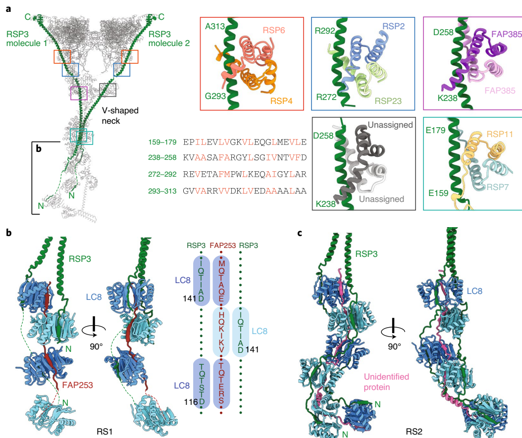
Fig. 4 | Interactions between RSP3 and radial spoke proteins. a , Left, atomic model of RS1 with its two molecules of RSP3 colored green. Colored boxes indicate the binding sites on RSP3 of five different dimers. The partially boxed proximal region of the stalk is shown in detail in b . Right, atomic models of the interactions between RSP3 and different dimers. The sequence alignment shows amphipathic helices of RSP3 with hydrophobic residues recognized by the various dimers colored red. The four-helix bundle of RSP7–RSP11 belongs to the RIIa dimerization/docking domain, and the four-helix bundles of RSP4–RSP6, RSP2–RSP23, RSP385–RSP385 and the unassigned dimer belong to Dpy-30 domain (which has an additional helix at the N-terminus as compared with the RIIa dimerization/docking domain). b , Left, orthogonal views of the interactions of RSP3 and FAP253 with the LC8 homodimers in RS1. Other subunits have been omitted for clarity. Right, a schematic showing the resolved LC8-binding motifs of FAP253 and RSP3. c , Orthogonal views of the interactions between RSP3 and the LC8 homodimers in RS2. An unassigned protein (pink) also interacts with the \beta -edges of LC8. Other subunits have been omitted for clarity.
