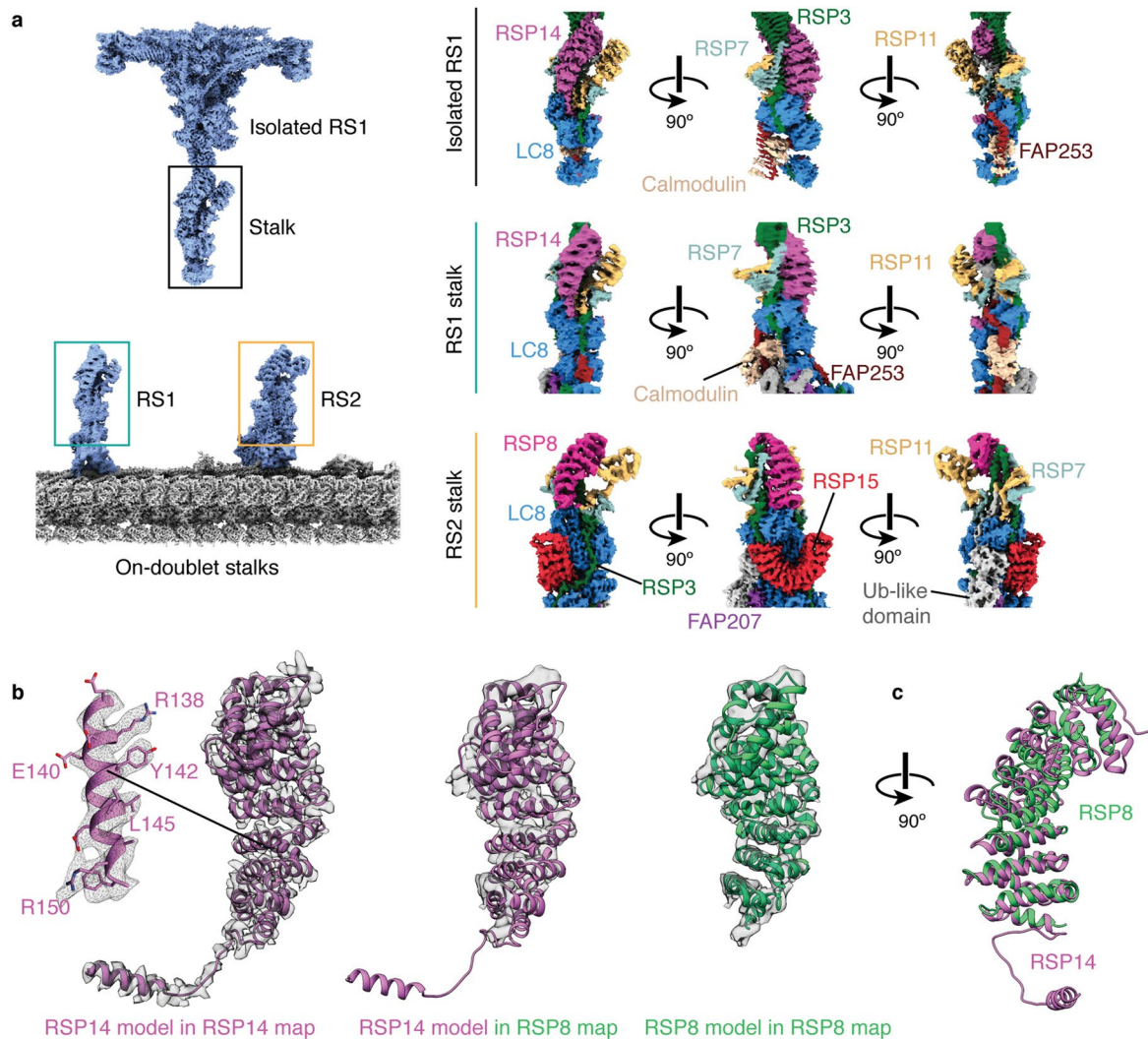
Extended Data Fig. 7 | The stalks of RS1 and RS2. a , The stalk of the isolated radial spoke is consistent with the on-doublet stalk of RS1 only. FAP253, RSP14, and calmodulin are present in the stalk of RS1 but not RS2. RSP8, RSP15, and an unidentified ubiquitin (Ub)-like domain are present in the stalk of RS2 but not RS1. LC8, FAP207, and RSP3 are common to both RS1 and RS2 but adopt different conformations. The RSP7/11 heterodimer is similar in both radial spokes. b , RSP14 and RSP8 are structurally similar armadillo proteins present in different radial spokes. Left, RSP14 was identified in the stalk of RS1 based on well-defined sidechain density. Middle, the model of RSP14 is incompatible with the density of the armadillo protein in RS2, indicating that they are different proteins with similar folds. Right, a model for RSP8 built into the RS2 density. c , Superposition of the atomic models for RSP8 and RSP14.
