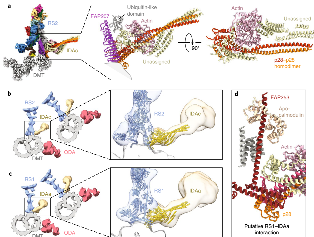
Fig. 5 | IDA subforms a and c dock onto the bases of radial spokes. a , Left, composite map showing the densities for the base of RS2, IDAc and the DMT. The maps of RS2 and IDAc are colored by subunit. Right, atomic model of IDAc showing the interaction with FAP207 and an unidentified ubiquitin-like domain of RS2. The unassigned helices of IDAc may correspond to the tail of the dynein heavy chain. b , Left, slice through the subtomogram average of the Chlamydomonas axoneme (EMD-6872), with RS2 colored blue, IDAc colored yellow, the ODA colored red and the DMT colored gray. Zoomed-in view showing the models of RS2 and IDAc (colored blue and yellow, respectively) docking into the subtomogram average. c , Left, slice through the subtomogram average of the Chlamydomonas axoneme (EMD-6872) with RS1 colored blue, IDAa colored yellow, the ODA colored red and the DMT colored gray. Zoomed-in view showing the atomic models of RS1 and IDAa (colored blue and yellow, respectively) docking into the subtomogram average. The putative interface between IDAa and RS1 is distinct from the interface between RS2 and IDAc. d , Details of the expected interface between RS1 and IDAa based on docking the model of IDAc into the subtomogram average map of IDAa (EMD-6872).
