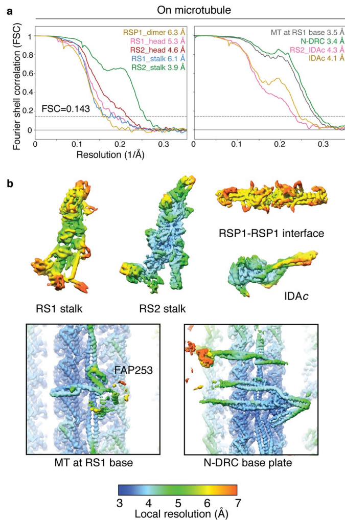
Extended Data Fig. 2 | Global and local resolution of on-doublet complexes. a , Fourier shell correlation (FSC) curves calculated between masked independent half maps for on-doublet structures. Left panel, FSC curves are shown for focused refinements of the RS1 spoke head and stalk, RS2 spoke head and stalk, and the RSP1-RSP1 dimer. Right panel, FSC curves for the base of RS1, the RS2-IDAc complex, IDAc, and the N-DRC baseplate. The nominal resolution was estimated using the FSC = 0.143 criterion (dashed line). b , Density maps for on-doublet structures colored by local resolution. Only the maps used for model building are shown. The local resolution is colored from 3 to 7 Å.
