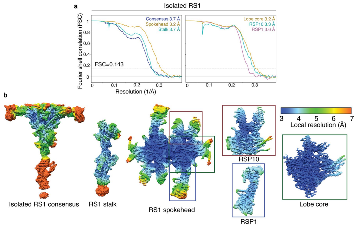
Extended Data Fig. 6 | Global and local resolution of isolated RS1. a , FSC curves calculated between masked independent half maps for isolated RS1. Left panel, FSC curves are shown for the consensus refinement of isolated RS1, focused refinement of the stalk, and focused refinement of the spoke head after applying C2 symmetry. Right panel, FSC curves for focused refinements of three subdomains of a single lobe of the RS1 spoke head. The colors of the curves match the masks used in Extended Data Fig. 5g. The nominal resolution was estimated using the FSC=0.143 criterion (dashed line). b , Density maps for the consensus refinement of isolated RS1 and various focused refinements colored by local resolution. The local resolution is colored from 3 to 7 \text{\AA} .
