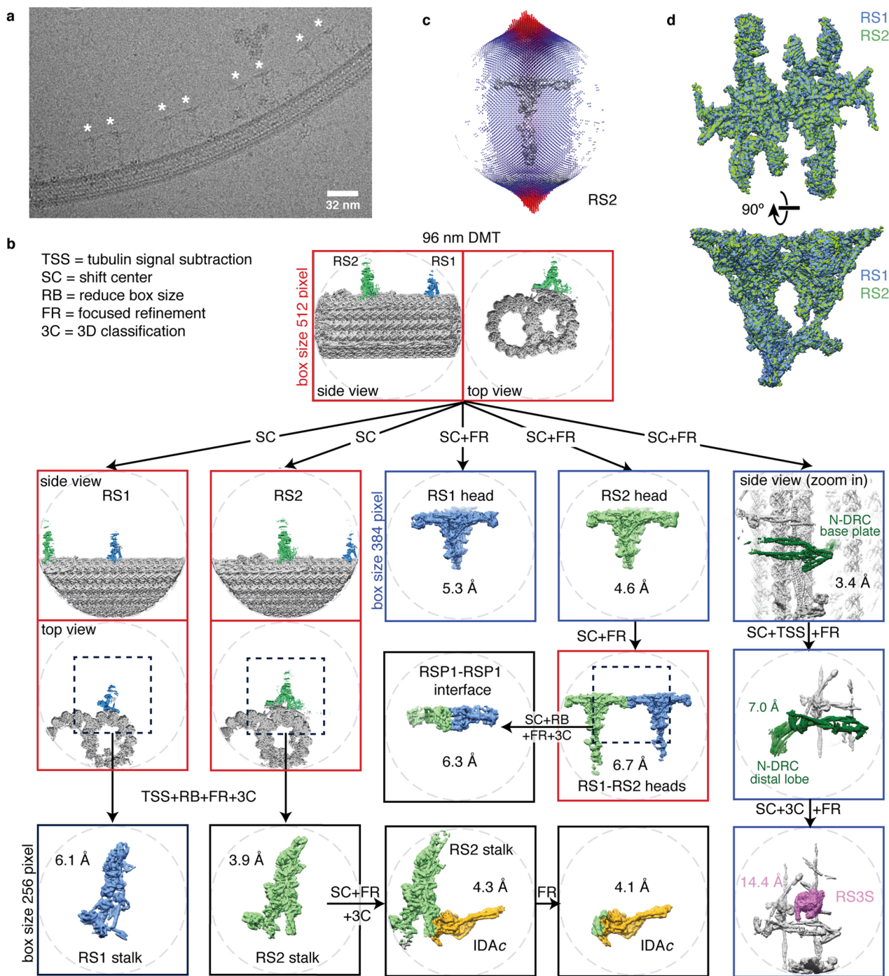
Extended Data Fig. 1 | Data collection and processing for the on-doublet complexes. a , Section of an electron micrograph showing radial spokes (marked with an asterisk) bound to a doublet microtubule in vitreous ice. b , Processing scheme used to generate reconstructions of complexes bound to doublet microtubules (DMT, gray). To resolve various structural features with 96-nm periodicity (RS1 spoke head/stalk, RS2 spoke head/stalk, RSP1-RSP1 interface, RS3S, IDAc, or N-DRC baseplate/lobe), it was necessary to use a combination of tubulin signal subtraction (TSS), shifting the center (SC) of coordinates to the feature of interest, focused refinement (FR) and 3D classification without alignment (3C). When possible, the box size was reduced (RB) to 256 or 384 instead of 512 pixels to facilitate data processing. c , Angular distribution of the particle views used for reconstruction of on-doublet RS2. Similar distributions were obtained for on-doublet RS1. The height of the cylinders, colored from blue to red, represents the number of particles. The final density map of RS2 is shown in gray. d , Superimposition of the on-doublet RS1 and RS2 spike heads confirms that they have identical structure.
