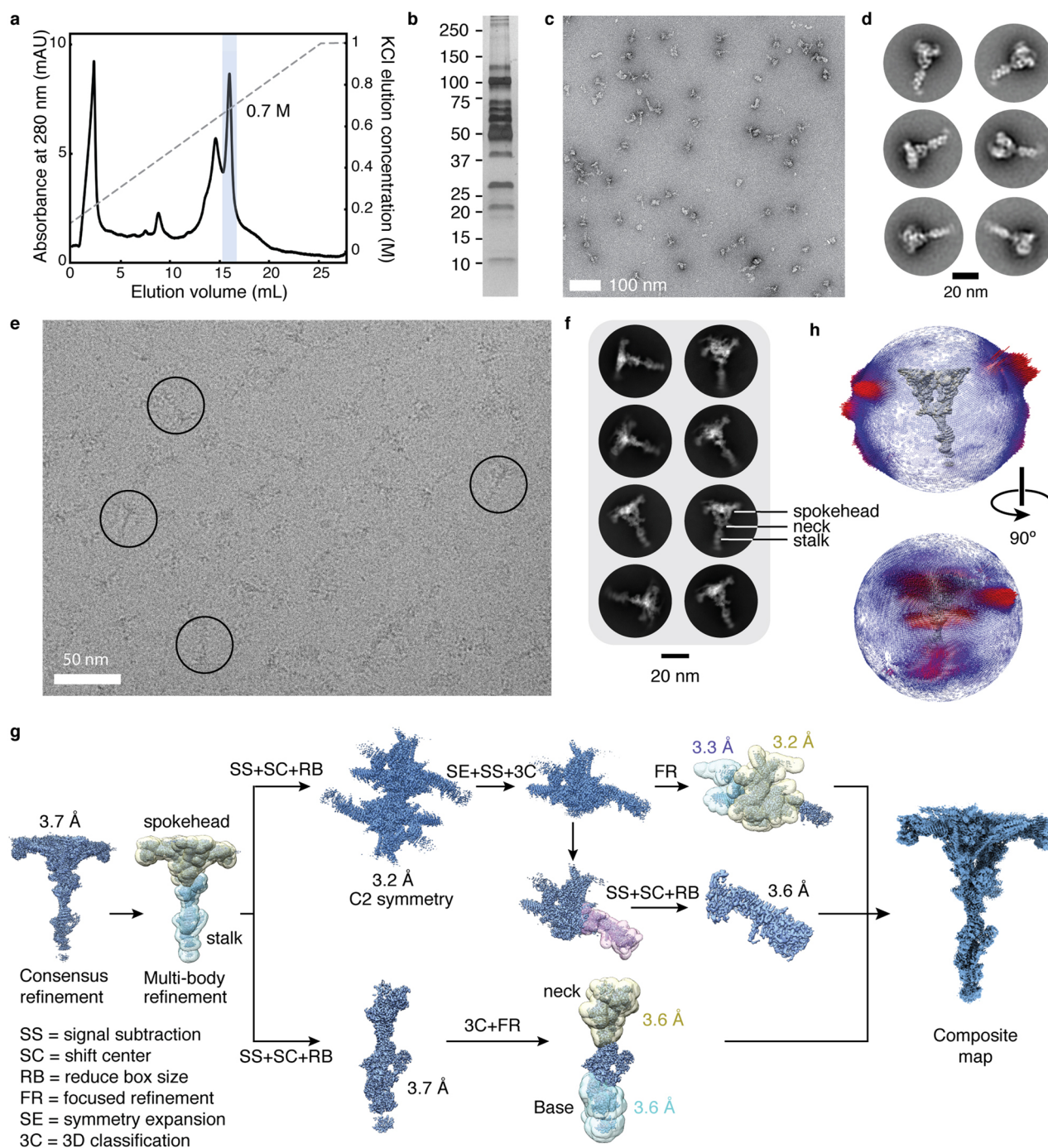
Extended Data Fig. 5 | Data collection and processing for isolated RS1. a , Chromatogram showing the elution of RS1 from an anion-exchange column using a KCl gradient. The peak fraction containing RS1 is highlighted and elutes at ~0.7 M KCl. b , Silver-stained SDS-PAGE gel showing the purity of isolated RS1 following anion-exchange chromatography. The molecular weights of markers (in kDa) are indicated on the left. The result of mass spectrometry analysis of this sample is given in Supplementary Data 1. c , Section of a negative-stain electron micrograph showing homogeneous and monodisperse radial spokes. d , Selected two-dimensional class averages of particles selected from negative-stain electron micrographs. e , Section of an electron micrograph showing radial spokes in vitreous ice. Particles showing the characteristic T-shaped projection of radial spokes are circled. f , Selected two-dimensional class averages of radial spokes showing well defined spoke heads but nebulous density for the stalk consistent with flexibility at the neck. g , Schematic showing the processing of the isolated RS1 data. Following a consensus refinement, the spoke head and stalk were independently refined. The twofold rotational symmetry of the spoke head was exploited to improve the map quality. Further masked refinement was used to improve the flexible projections of the spoke head and the base and neck of the stalk. These individual maps were recombined to generate a final composite cryo-EM map. h , Angular distribution of the particle views used for the consensus reconstruction of isolated RS1. The height of the cylinders, colored from blue to red, represents the number of particles. The final density map of RS1 is shown in gray.
