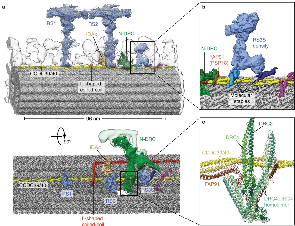
Extended Data Fig. 4 | Single-particle cryo-EM maps docked into a subtomogram average of the axoneme. a , Two views showing the single-particle cryo-EM maps of RS1, RS2, RS3S, N-DRC, and IDAc docked into the subtomogram average of the 96-nm repeat of the Chlamydomonas axoneme (EMD-6872). The subtomogram average is shown as a gray isosurface. b , Zoom-in view showing the map of RS3S. Density for RS3S is recovered in 25% of the particles following 3D classification (Extended Data Fig. 1b). RS3S interacts with two molecular staples of unknown identity. c , Zoom-in view showing the model and map for the N-DRC baseplate. Three N-DRC subunits (DRC1, DRC2, and DRC4) can be unambiguously identified. FAP91 interacts with all three.
